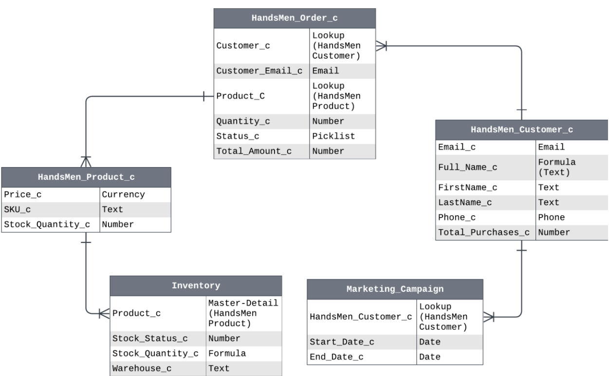
Fig. 1. Entity Relationship Diagram of HandsMen Threads
